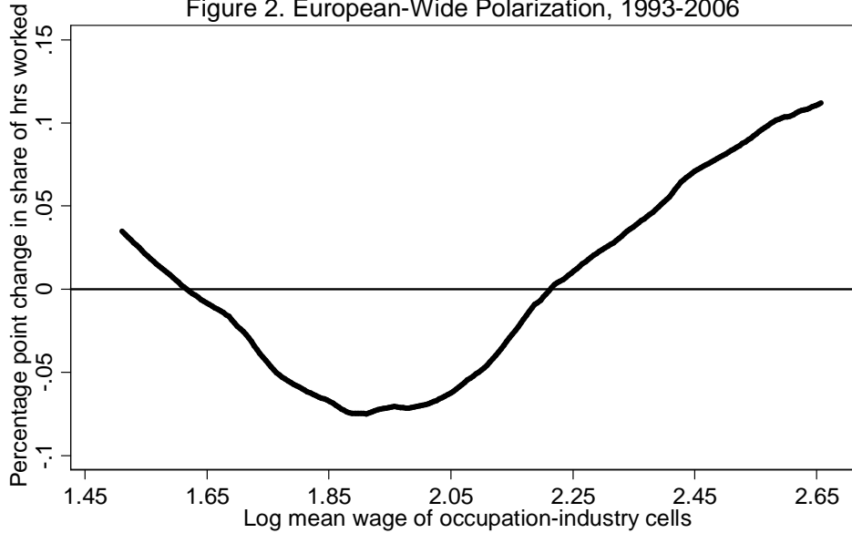
Figure 2. European-Wide Polarization, 1993-2006
