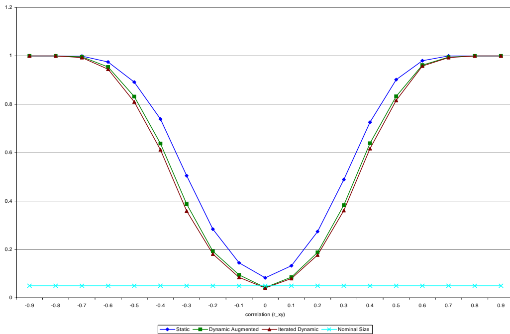
Figure 2. Power Curves for Maximum Canonical Correlation Test ( \varphi = 0.5, m = 2, T = 100 )
